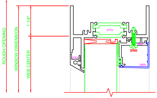
100 HEAD SERIES: 321G FIXED
