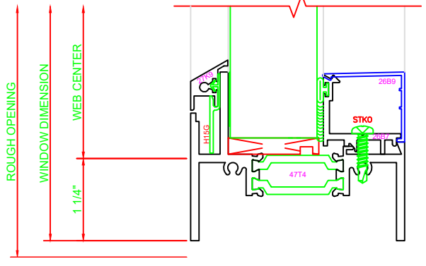
200 SILL SERIES: 321G FIXED
